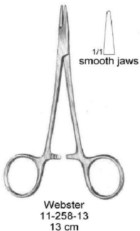
A001362/ 11-258-13 Porta agujas Webster 13cm
